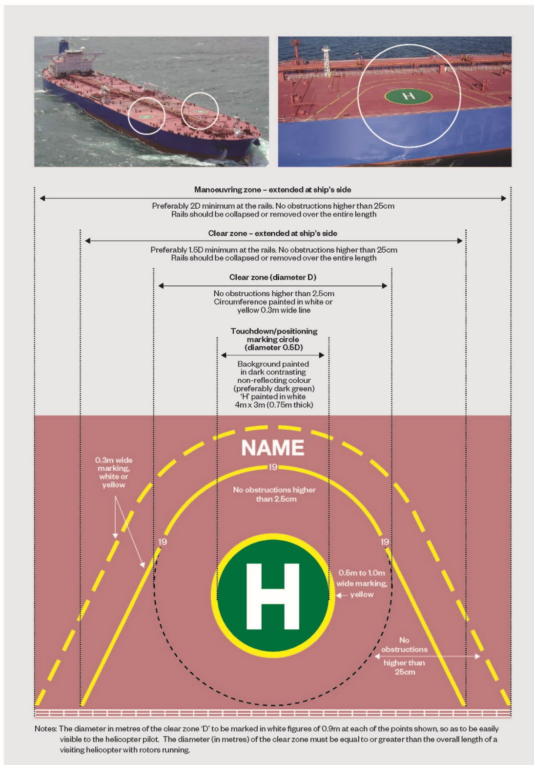
Figure 4: Ship's side non-purpose-built landing area markings 3
