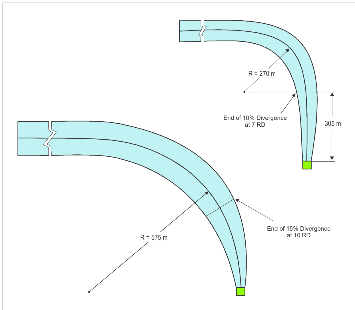
Figure 4-1. Curved approach and take-off climb surface for all FATOs
