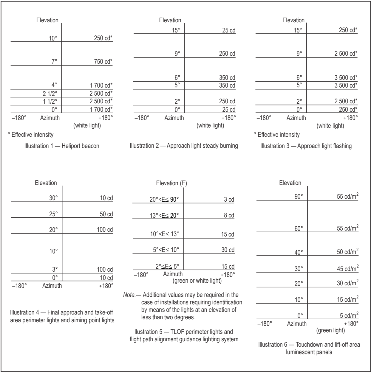
Figure 5-12. Isocandela diagrams
