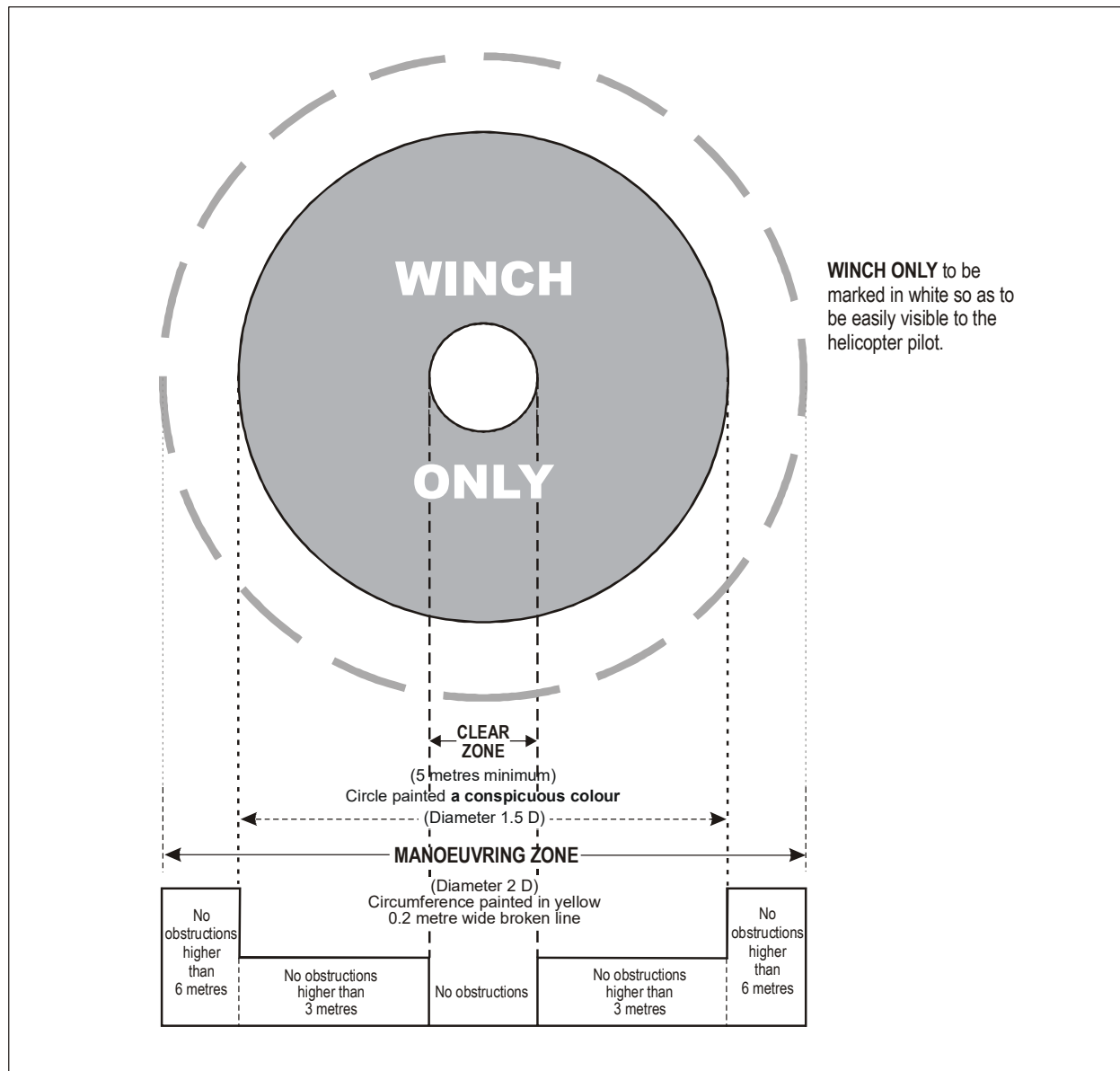
Figure 4-7. Winching area of a ship
